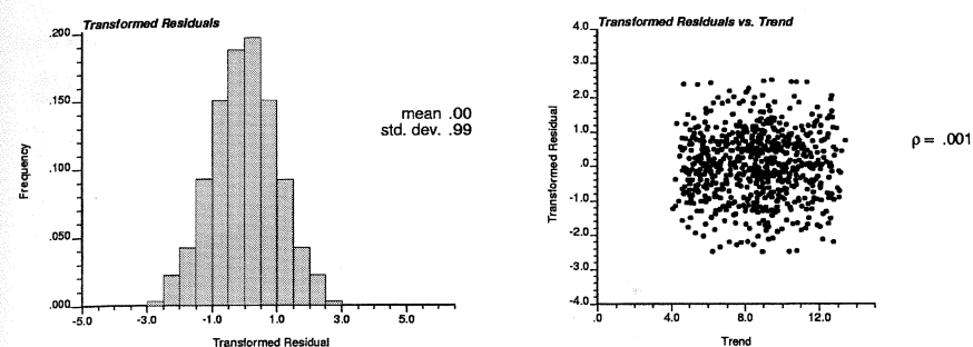
Figure 8. Histogram of transformed residual (left) and crossplot of normal score transformed trend vs. the conditionally transformed residual components.
