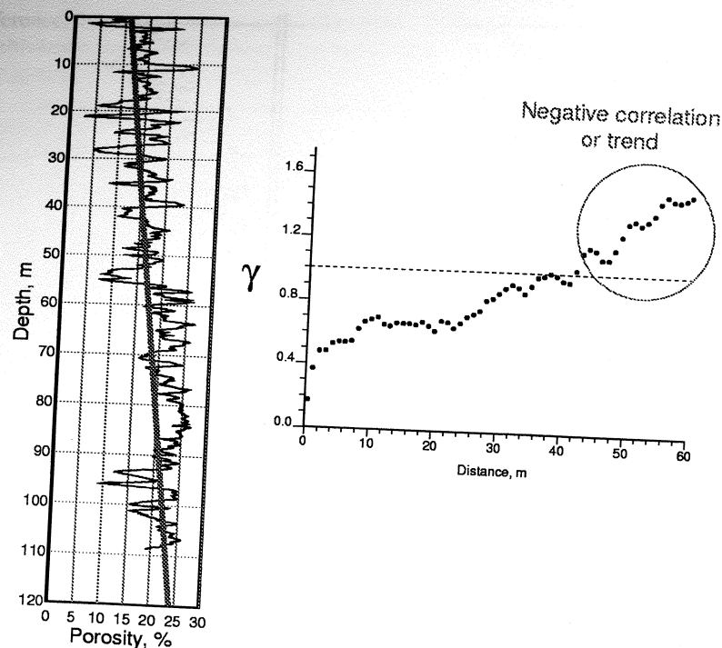
Figure 2. Example of porosity log (left) and corresponding vertical variogram (right) showing existence of a vertical trend.
